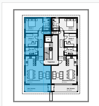
Attikageschoss Haus B
